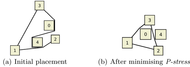
Fig. 3. Example of how our layout algorithm improves the network layout by reducing P -stress (which shortens edge routes) while preserving the topology of the initial layout.
