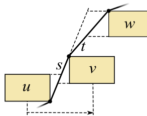
Fig. 4. Constraints generated during a vertical scan. There is one separation constraint x_u + \frac{1}{2}(\text{width}(u) + \text{width}(v)) \leq x_v to prevent overlap, three bend constraints (the construction for the constraint ensuring the path remains tight around v is shown) and three straight constraints at the places where the segments s and t may potentially bend.
